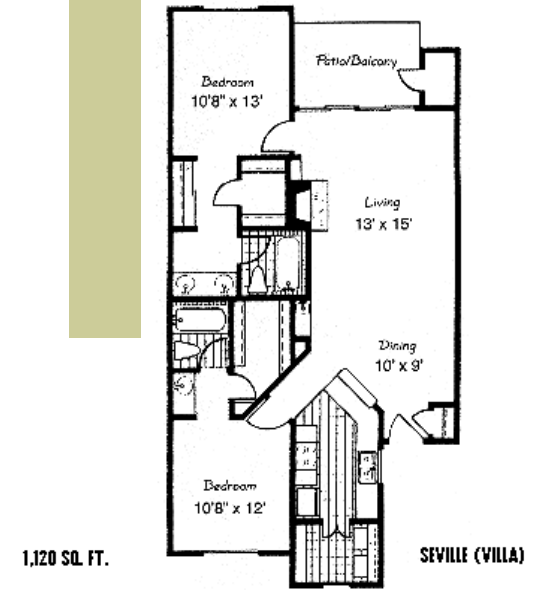
2 Bedroom 2 Bath Single Story Villa
